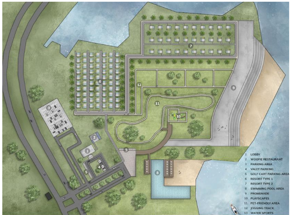
Lampiran 1. Site Plan
