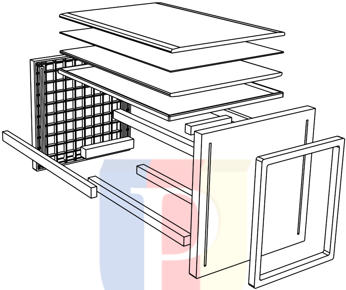
Lampiran 24 Exploded View Modul Utama
