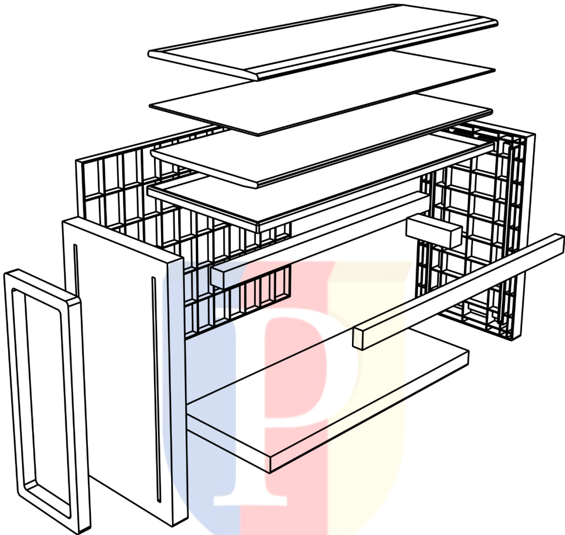
Lampiran 25 Exploded View Modul Tambahan
