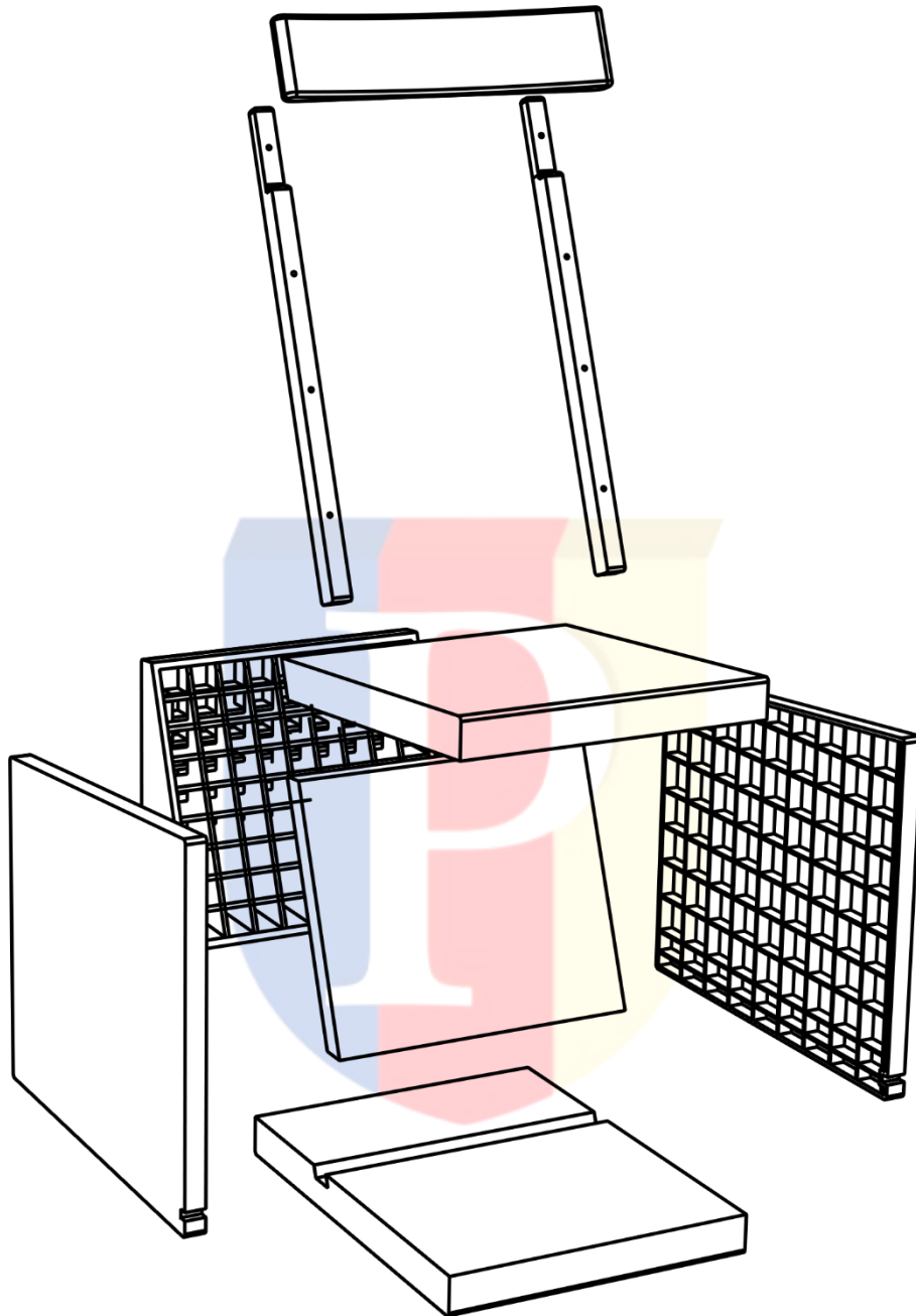
Lampiran 26 Exploded View Modul Kursi
