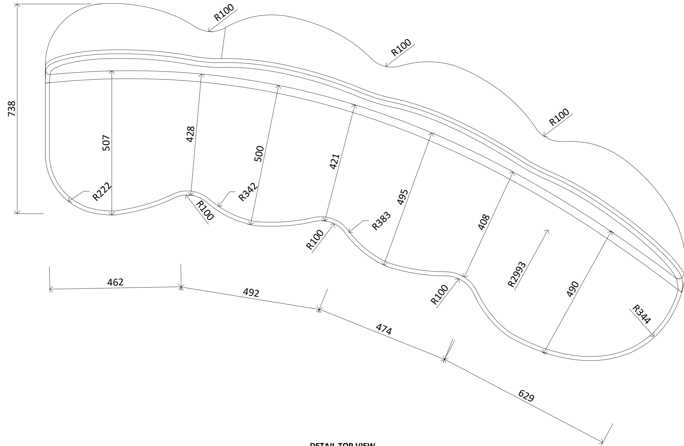
DETAIL TOP VIEW
